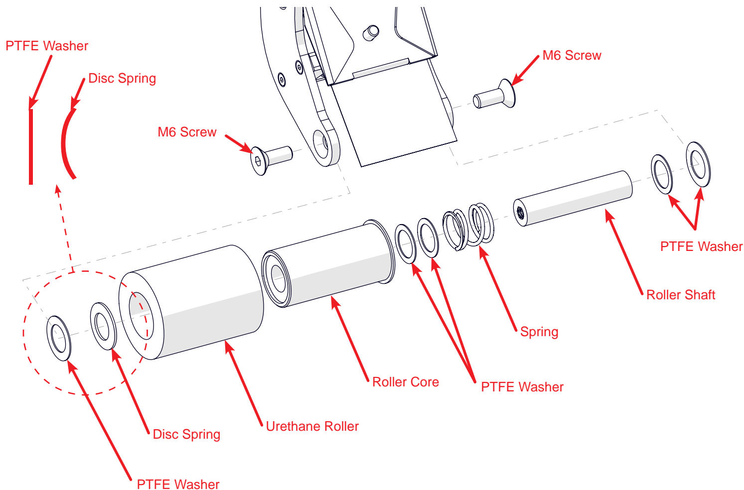
Figure 20: Front Roller Disassembly
