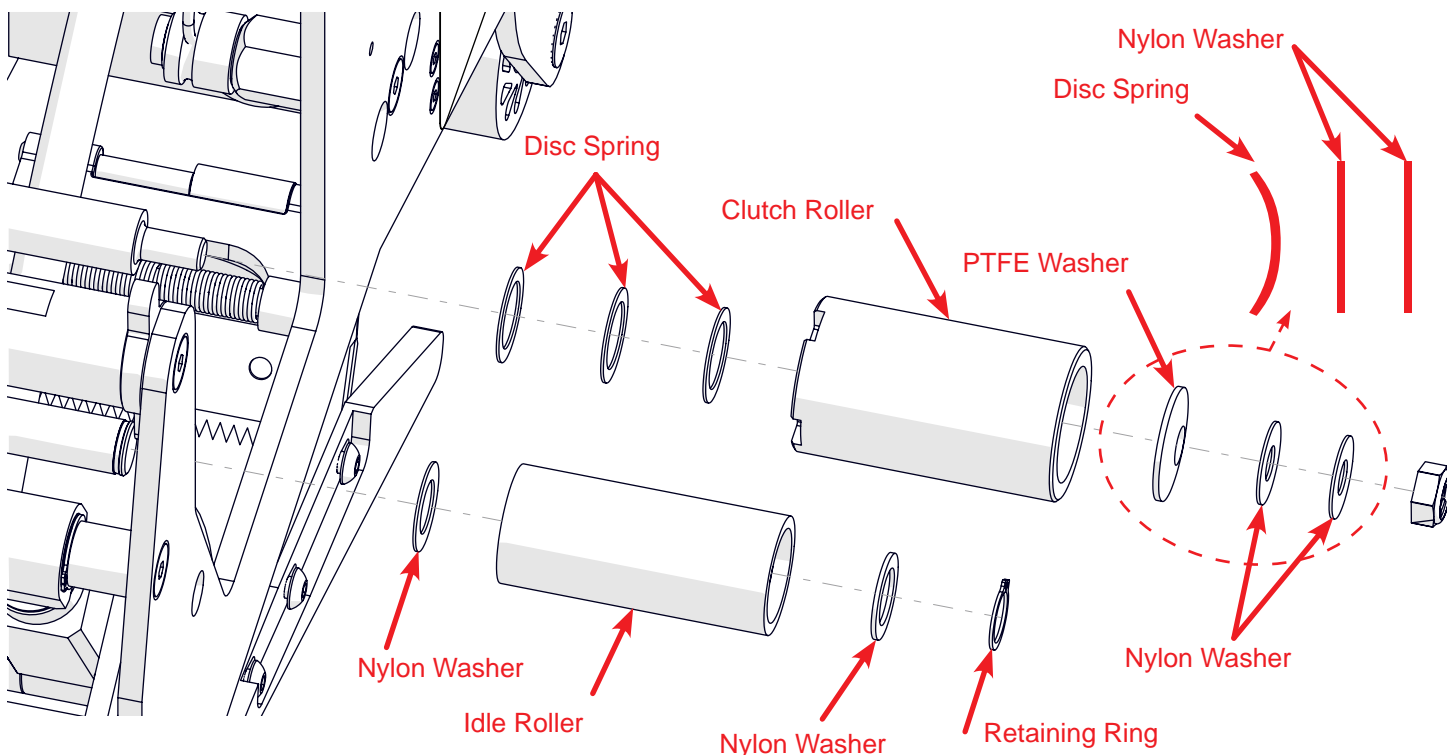
Figure 26: Removal and Disassembly of the Clutch Rollers
