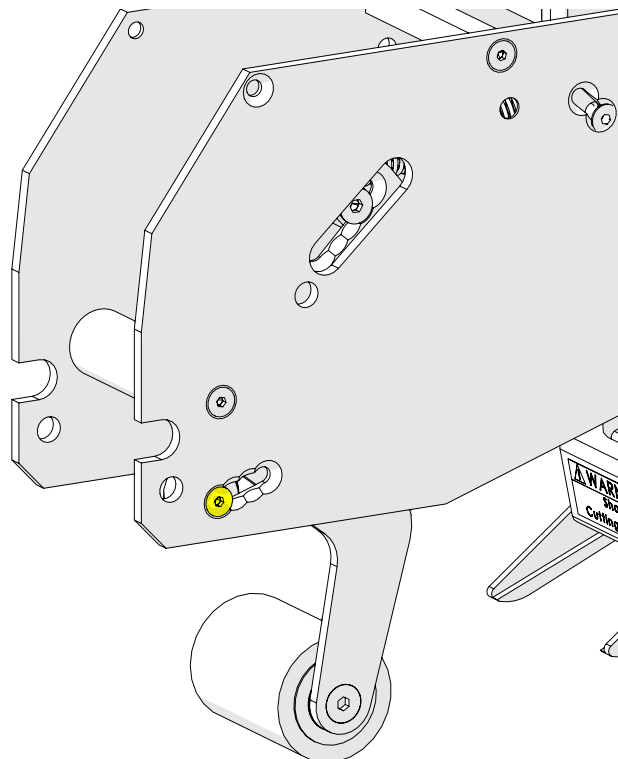
Figure 14: Low Profile Adjustment
