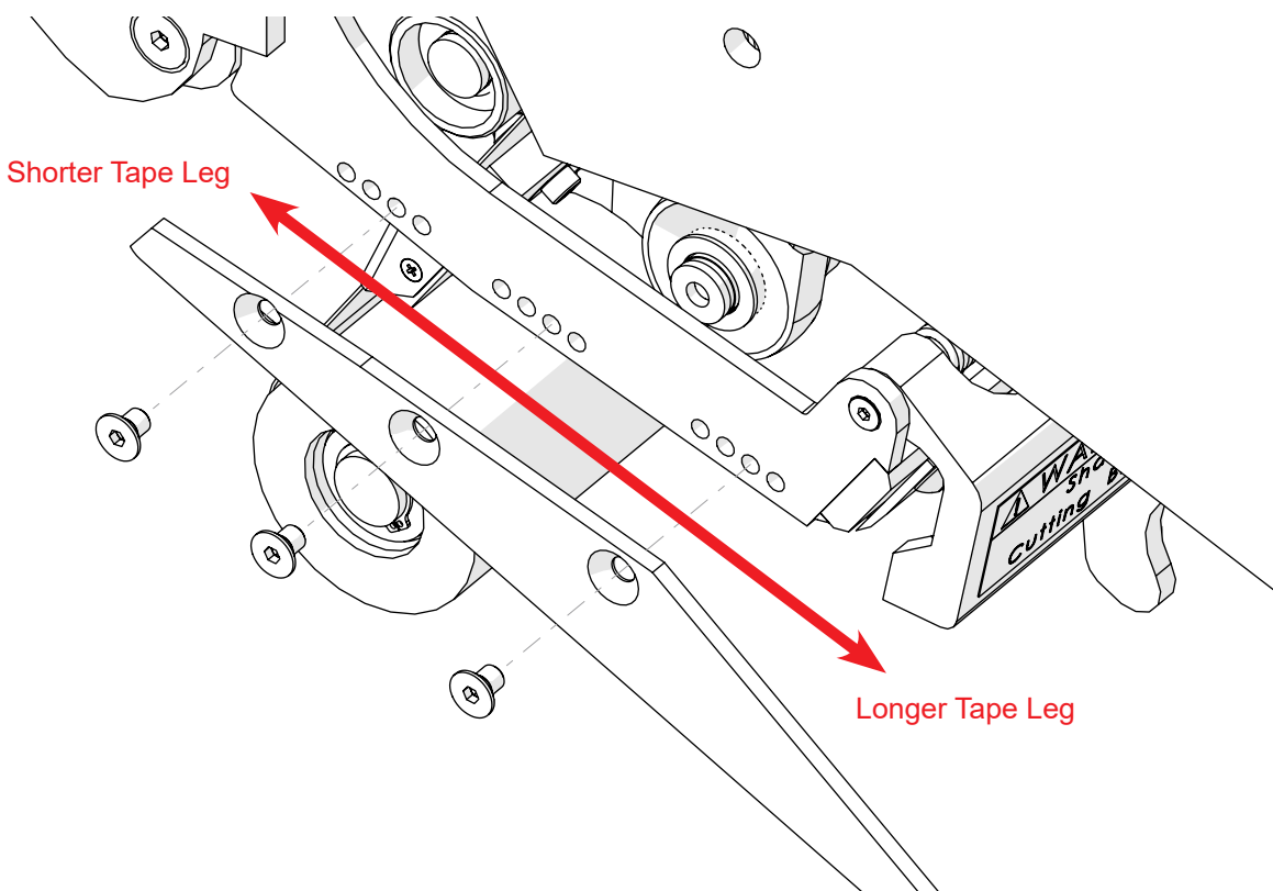
Figure 12: Rear Tape Leg Adjustment
