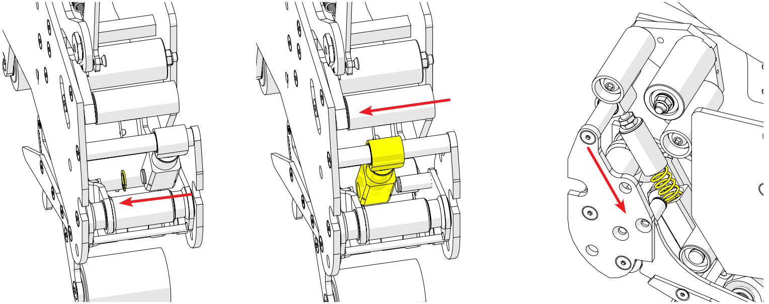
Figure 25: Replacing Knife Arm Spring
