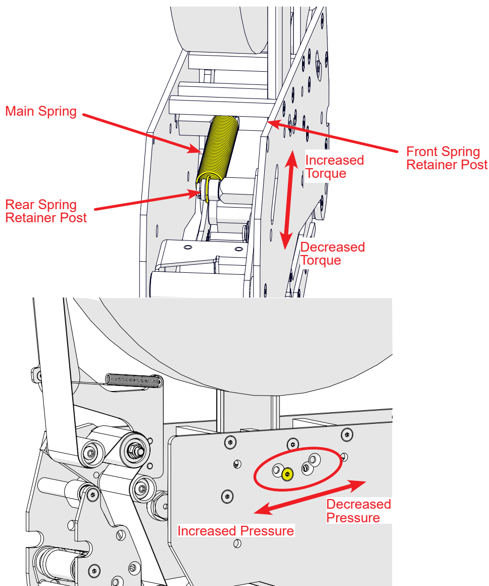
Figure 15: Main Spring Adjustments
