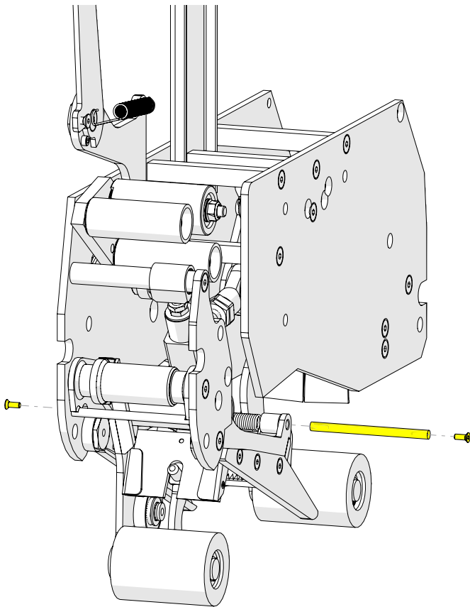
Figure 23: Removing Tape Guard Rod
