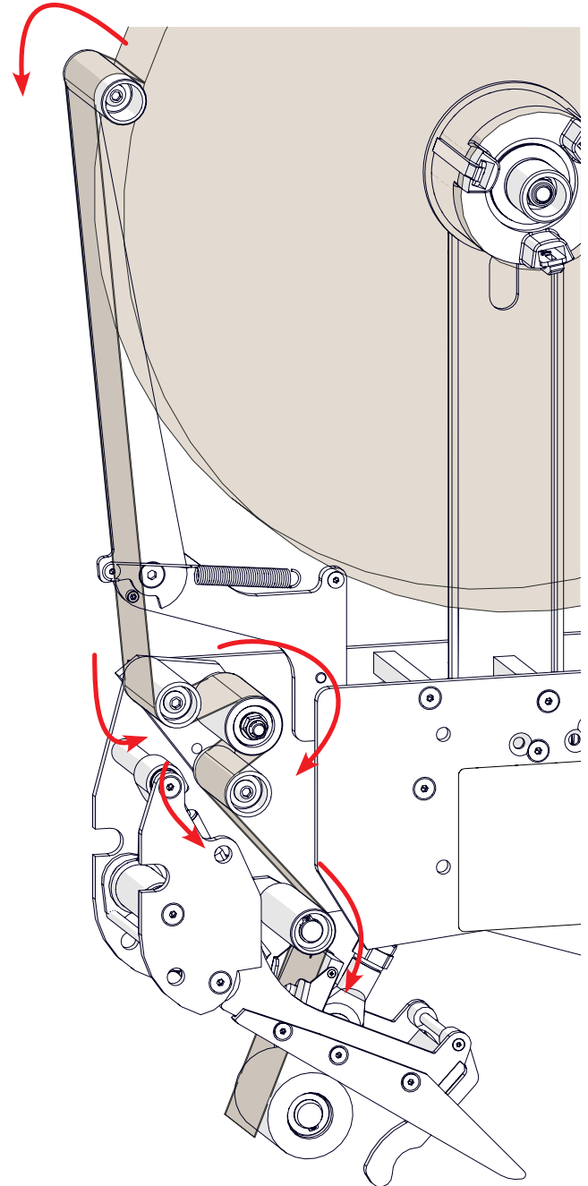
Figure 9: 3D Tape Path
