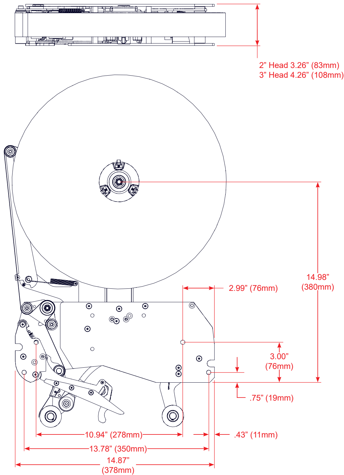
Figure 7: Dimensions
