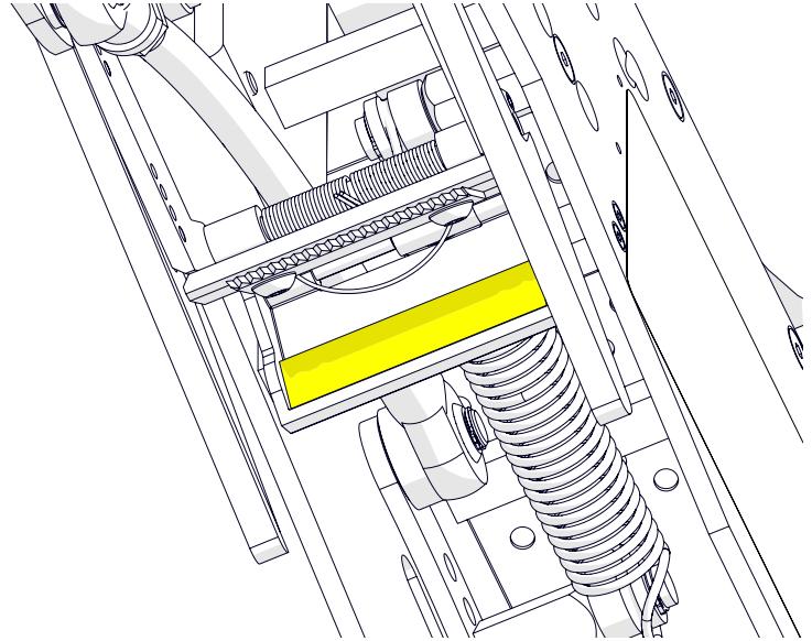
Figure 18: Oiler Pad
