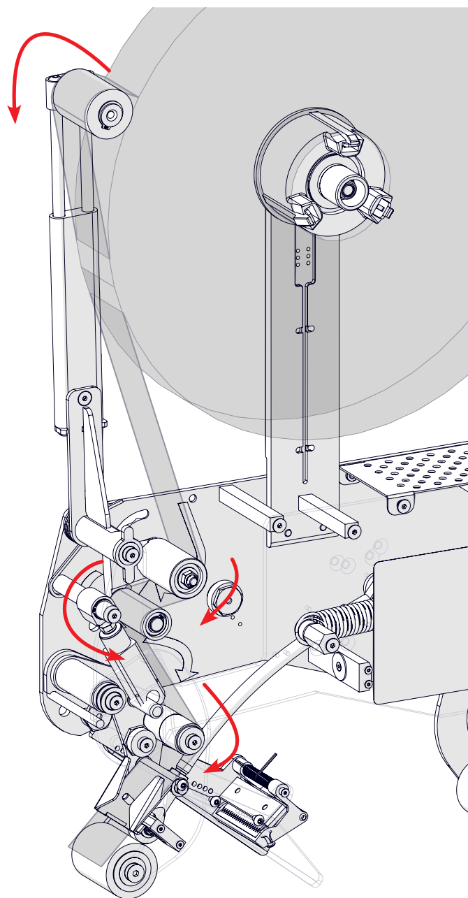
Figure 9: 3D Tape Path
