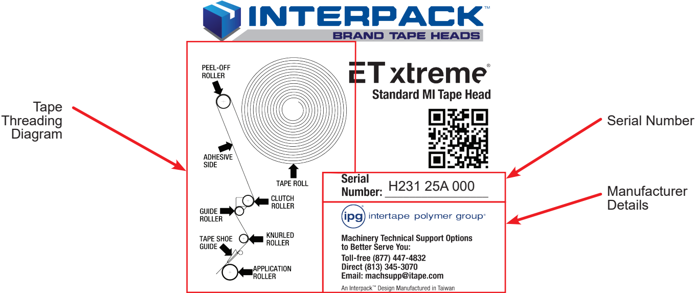
Figure 6: Label Identification
