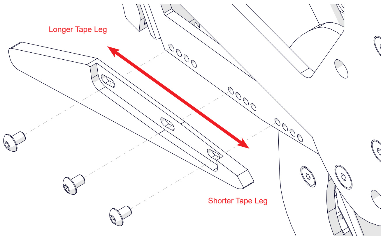
Figure 12: Rear Tape Leg Adjustment
