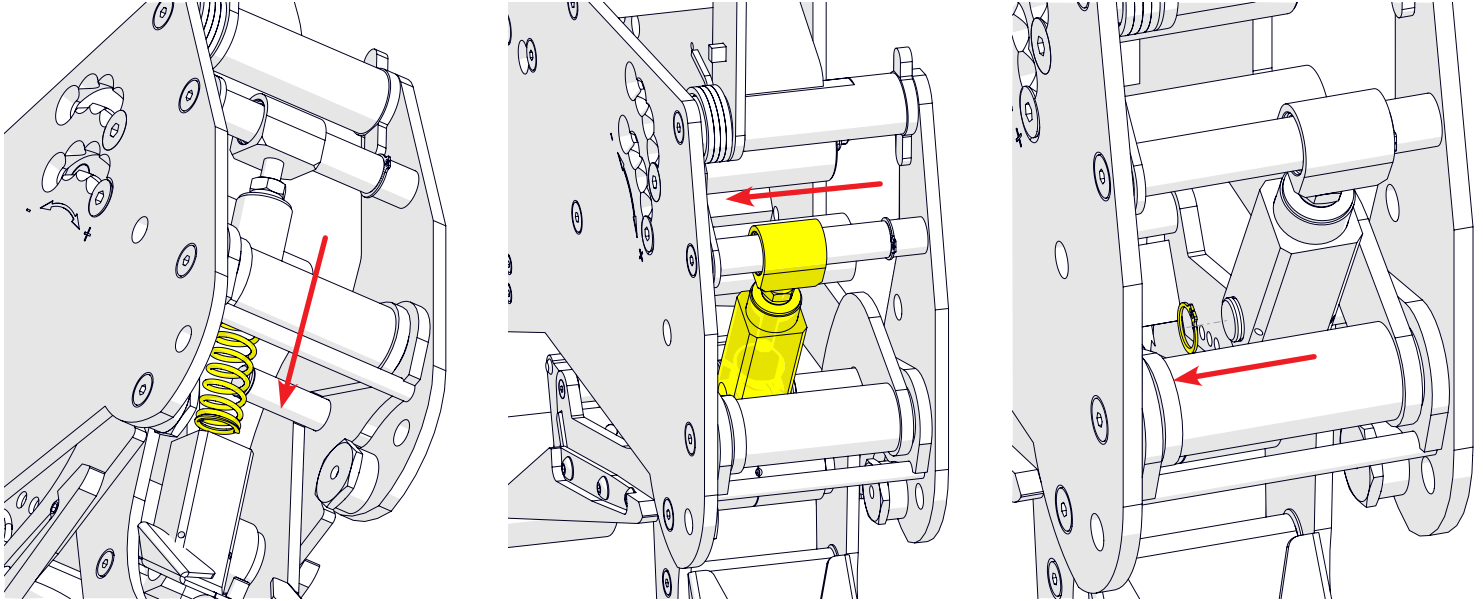
Figure 25: Replacing Knife Arm Spring
