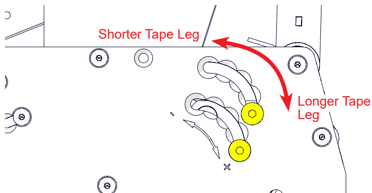
Figure 11: Front Tape Leg Adjustment
