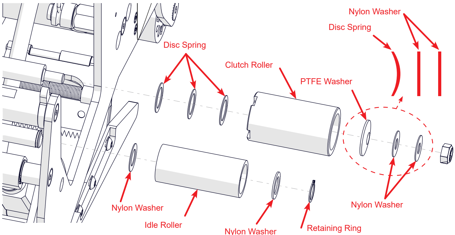
Figure 26: Removal and Disassembly of the Clutch Rollers
