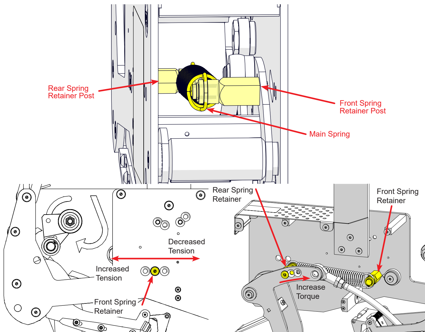
Figure 15: Main Spring Adjustments
