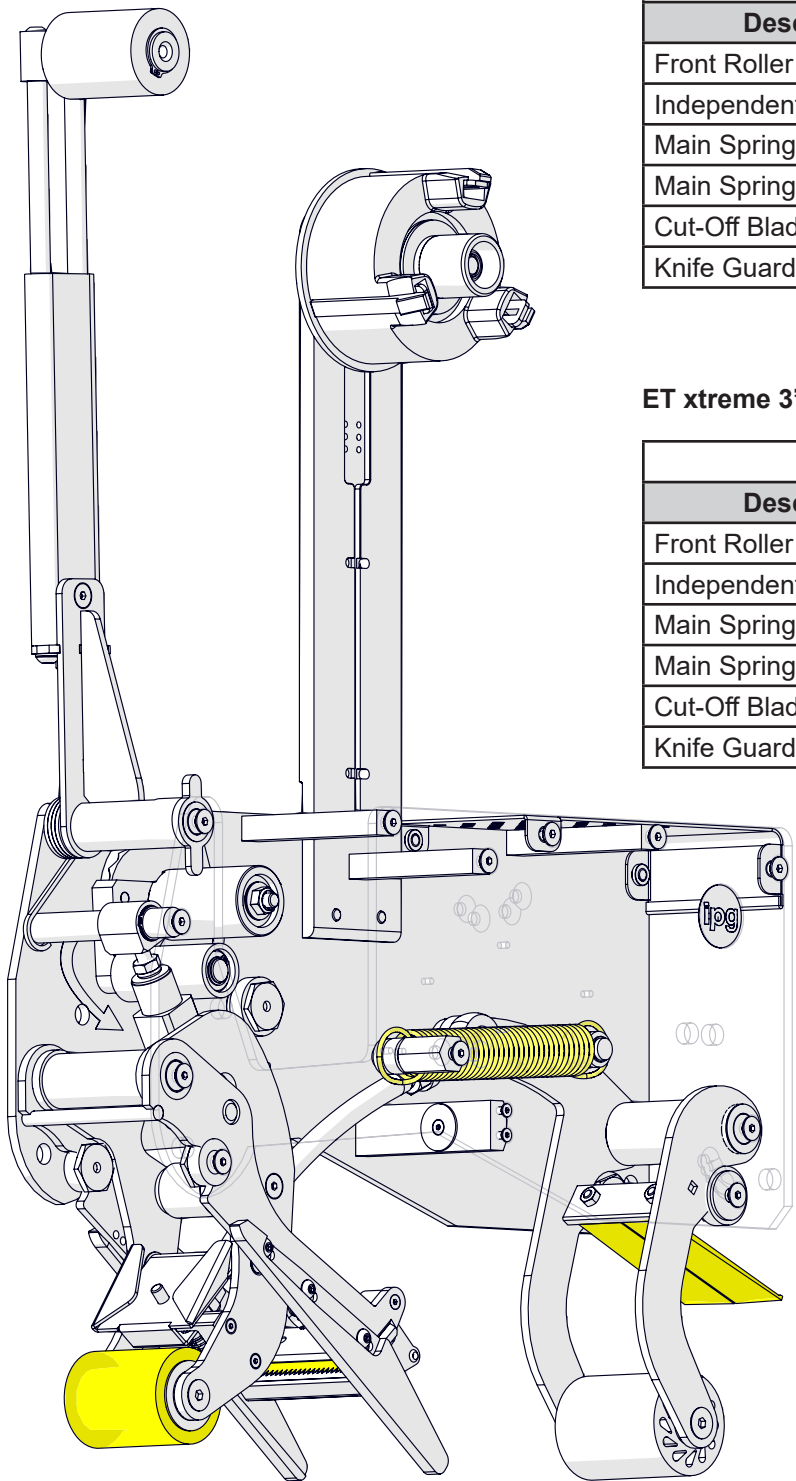
Figure 28: Spare Kit Components
