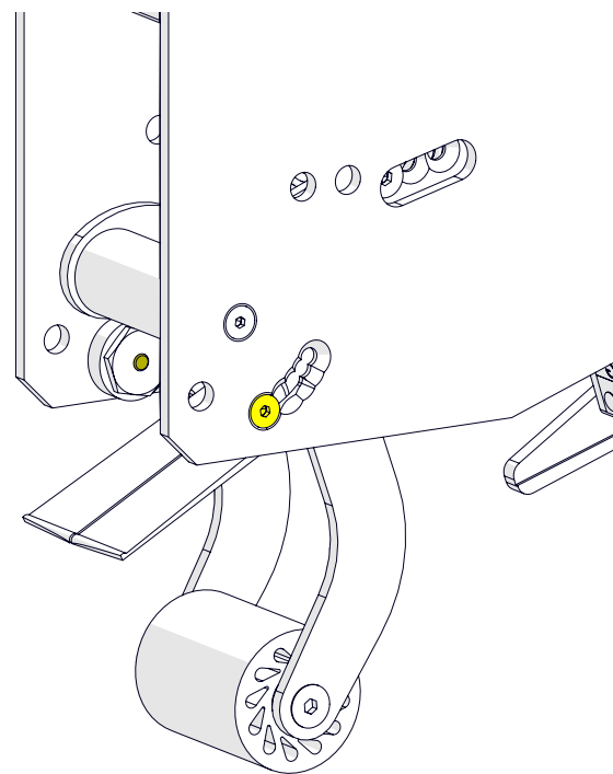
Figure 14: Low Profile Adjustment
