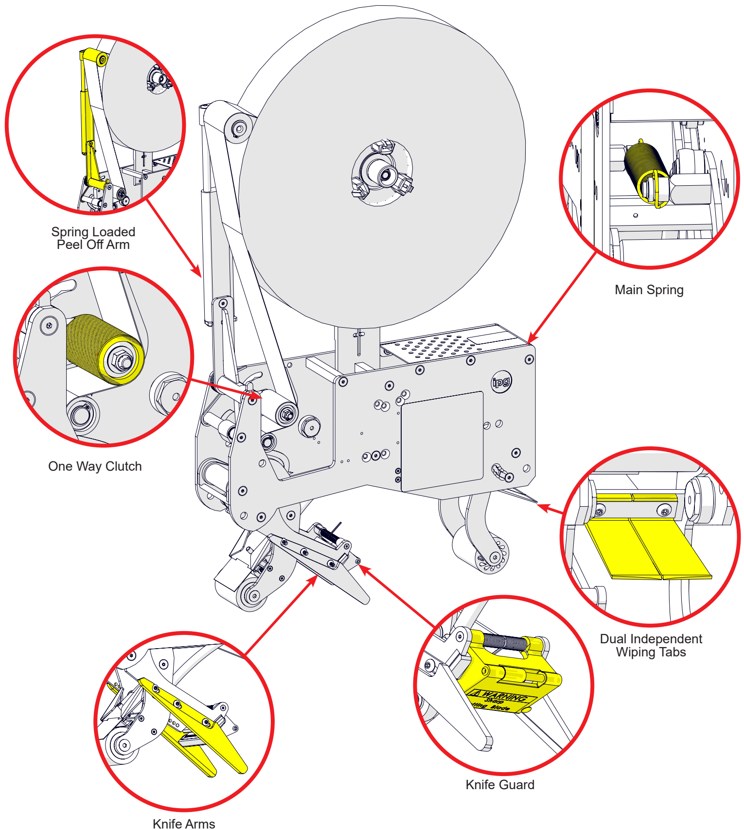
Figure 8: Components
