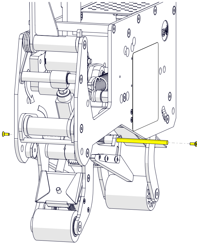
Figure 23: Removing Tape Guard Rod
