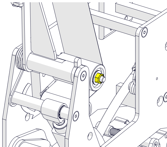
Figure 13: Clutch Adjustment
