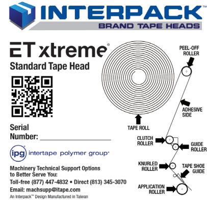
Figure 4: Serial Label
